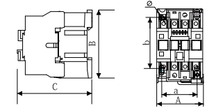
Figure 1: Outline and Installation Dimensions of CJX2-09~32 AC Contactor
