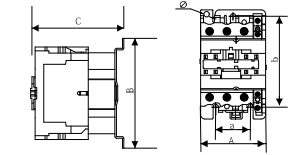
Figure 2: Outline and Installation Dimensions of CJX2-40~95 AC Contactor
