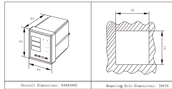
Overall Dimensions: 84*84*85
