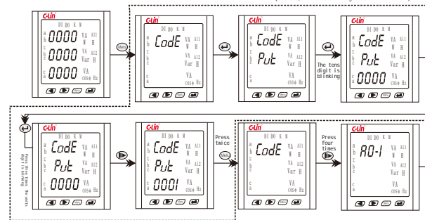
Example 3: Analog Transmitter Output Setting (Example: Set A01: Output a 4-20mA analog signal corresponding to phase B voltage (0-220V)).
