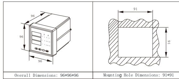
Overall Dimensions: 96*96*96
