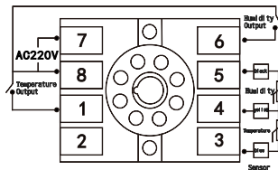
▲ Wiring Diagram for Dual-Load Product
