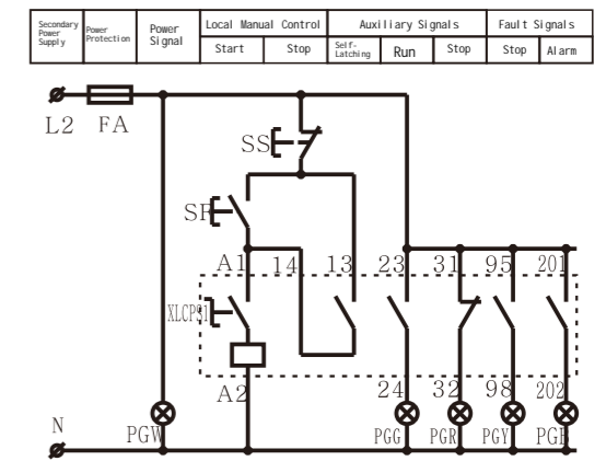
Manual Panel + Local Control
