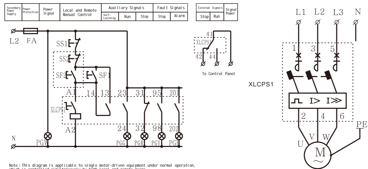
Manual Panel + Local Control + Remote Control
