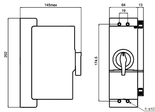
XLCPS1-45 Control and Protection Switch Device
