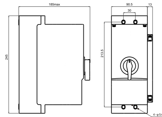
XLCPS1-125 Control and Protection Switch Device
